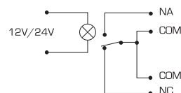
electrical connection
