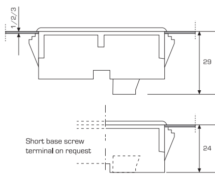
External RP63 Push Button Dimensions
